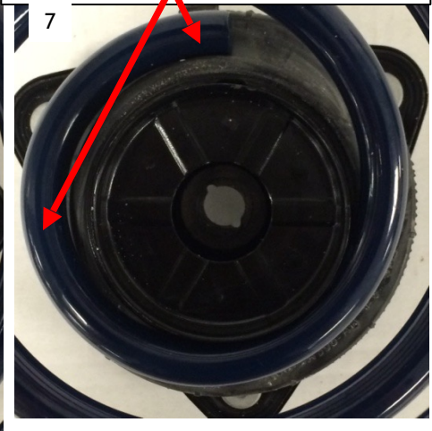
Incorrect, notice how the coil only wraps 1/4 of the way around the upper spring seat.
